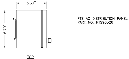
3 06 AC LOAD CENTER DETAIL NTS
