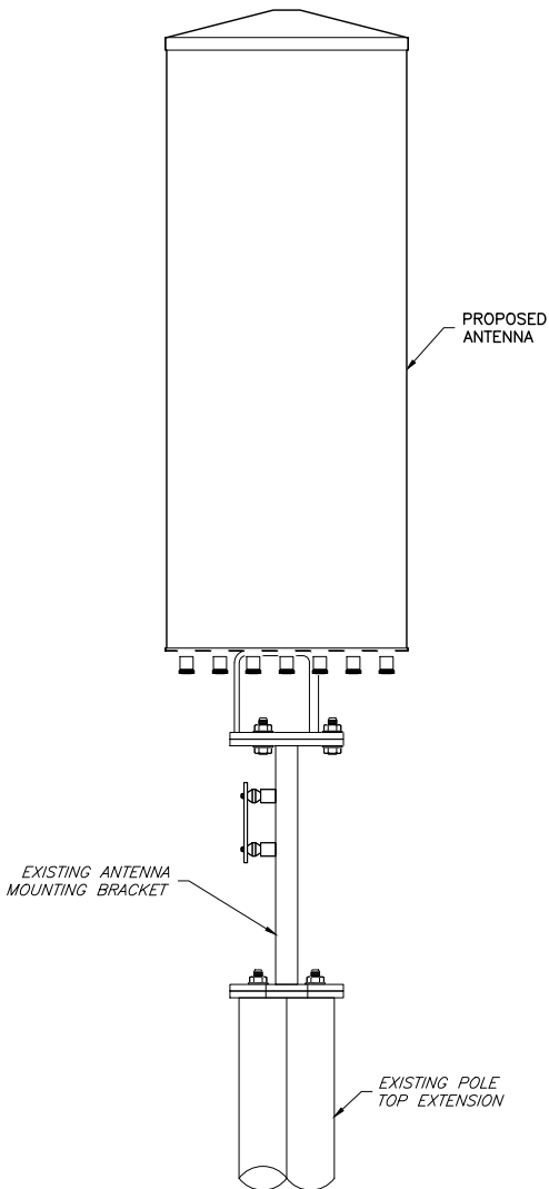
5 06 ANTENNA MOUNTING DETAIL NTS
