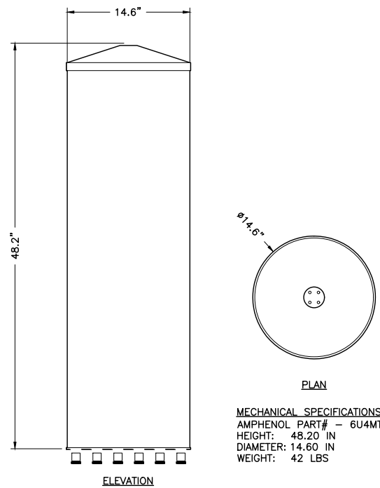
6 06 ANTENNA DETAIL NTS
